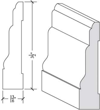
CAS-130 13/16" X 3-1/2"
